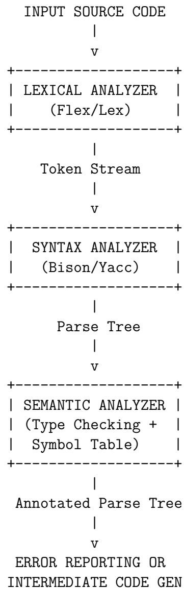
Figure 1: Compiler front-end architecture
